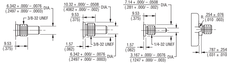
Anti-rotation Lug View
