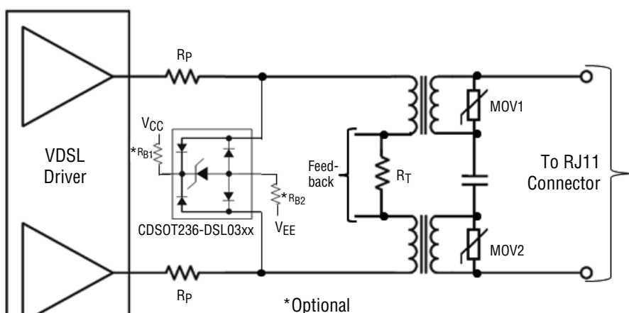
Figure 1. VDSL Driver Protection Design Topology
