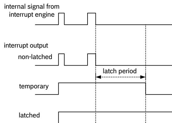
Figure 6: Interrupt modes
