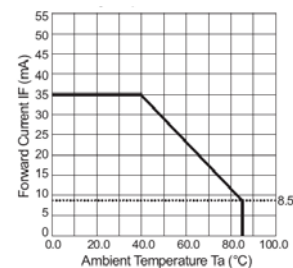
Derating Graph 4
