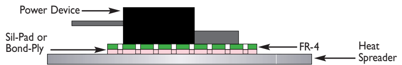
Mid Power Application with Bond-Ply
