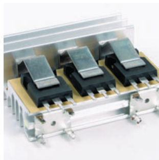
Choose a Sil-Pad that optimizes thermal performance for our mounting method — screw, clip, spring, bar, and so on.
