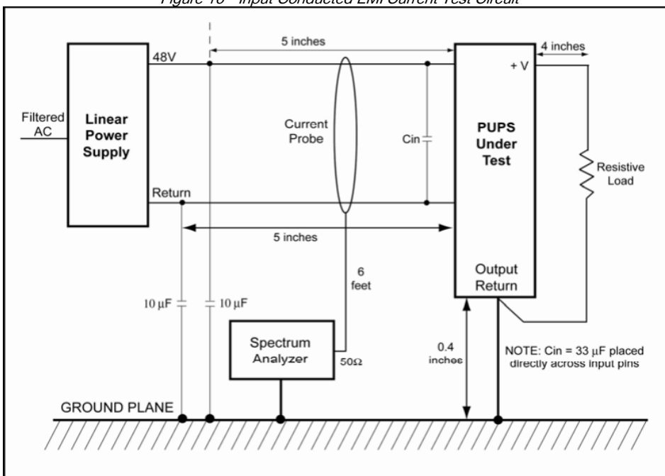
Figure 16 - Input Conducted EMI Current Test Circuit
