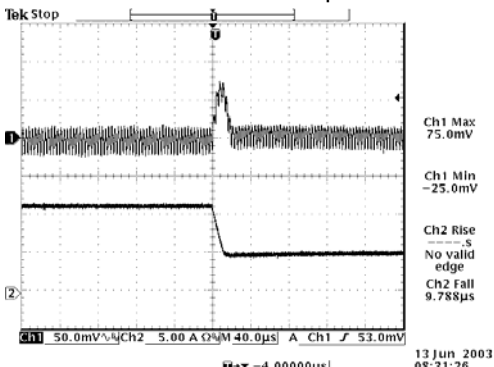
100% to 50% load 5 Vdc Input 1.5 Vdc Output
