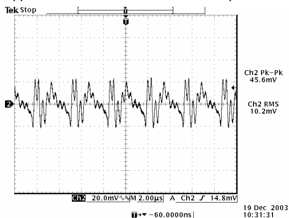
Ripple and noise at full load 1.5 Vdc output
