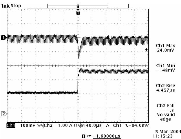
50% to 100% load Transient at Vin=5 V, Vo= 1.5 V
