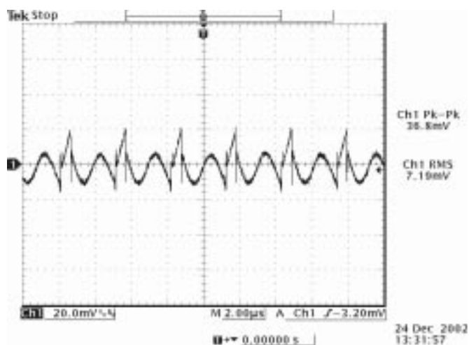
Ripple and noise at full load and 8Vdc input, 1.2Vdc output and Ta=25° C
