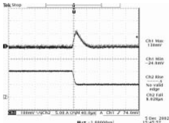
Vout=5.0V 100% to 50% load transients at 8V input and Ta=25° C
