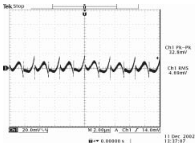
Ripple and noise at full load and 8Vdc input, 3.3Vdc output and Ta=25° C
