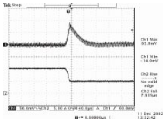
Vout=3.3V 100% to 50% load transients at 8V input and Ta=25° C
