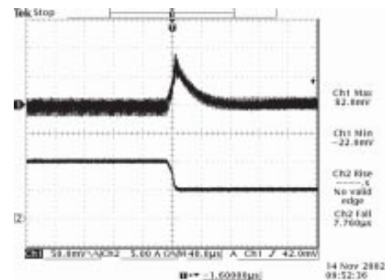
Vout=2.5V 100% to 50% load transients at 8V input and Ta=25° C
