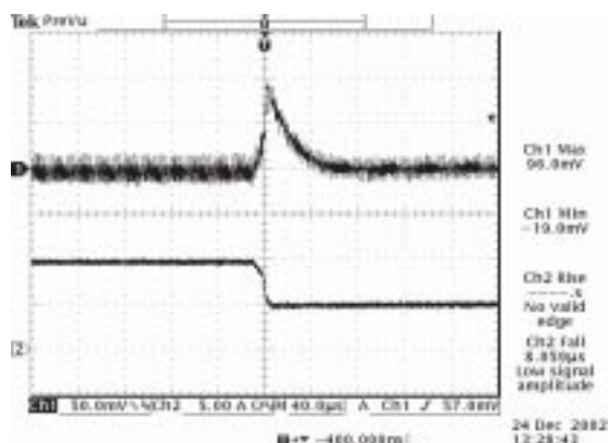
Vout=1.2V 100% to 50% load transients at 8V input and Ta=25° C
