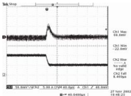
Vout=1.8V 100% to 50% load transients at 8V input and Ta=25° C
