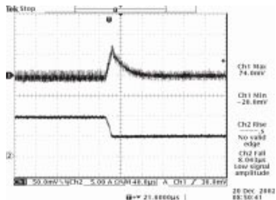
Vout=1.5V 100% to 50% load transients at 8V input and Ta=25° C
