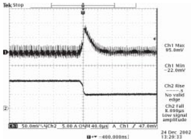
Vout=1.0V 100% to 50% load transients at 8V input and Ta=25° C
