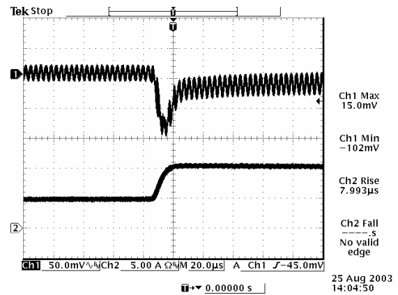
Transients 50% to 100% load 1.0 Vdc output
