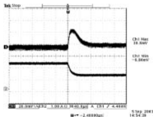
Vout=0.9V 100% to 50% load transients at 12V input and Ta=25° C
