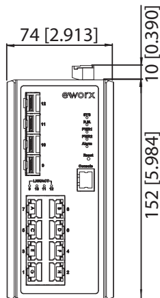
Model SEGP512-4SFP-T faceplate detail
