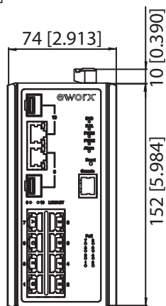
Model SEGP510-2SFP-T faceplate detail
