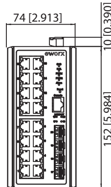
Model SE520-4SFP-T faceplate detail
