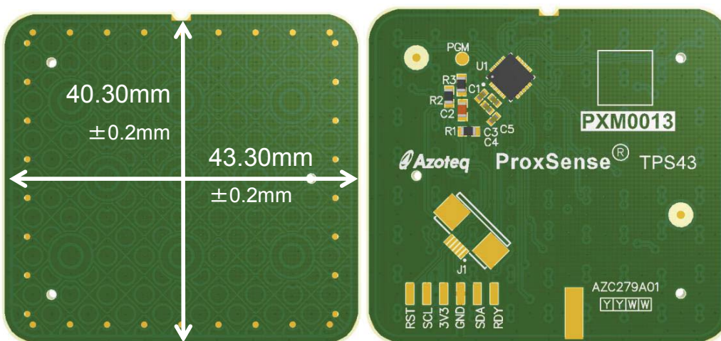
Figure 2.1 TPS43 – Module Representation
