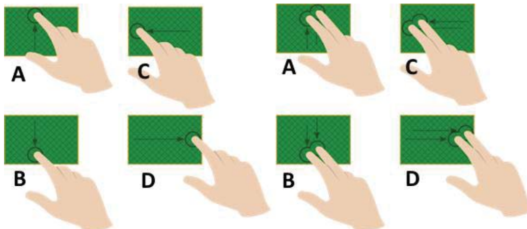
Figure 4.1 Swipe Gestures
