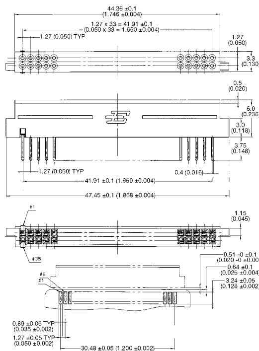
RECOMMENDED PCB PATTERN
