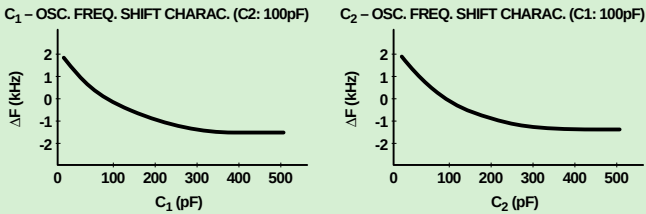
Figure 7: Load Capacitor Effects
