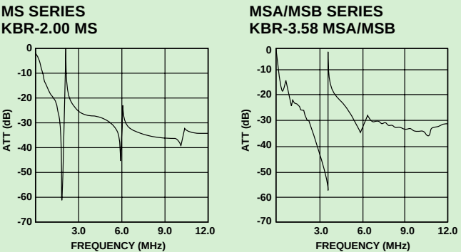
Figure 11: MHz Spurious Response
