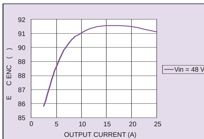
Figure 10 - Typical Efficiency vs. Output Current – RFF700-48S28Y
