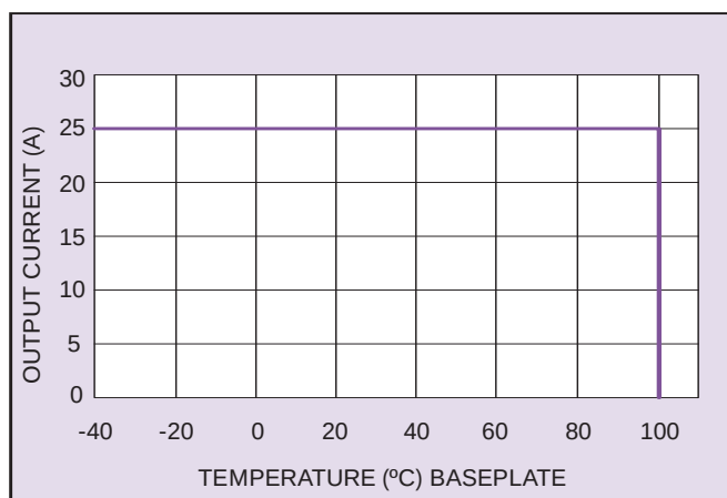
Figure 4 - RFF700 Derating Curve
