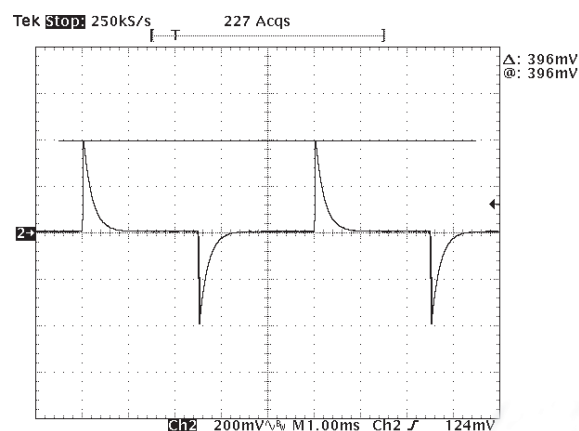
Figure 12 - RFF700-48S28Y Transient Response Load 12.5 A to 18.75 A
