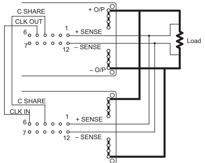
Parallel Connections
