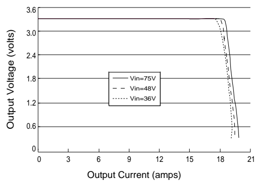
AV60A-048L-033D025(N) Typical Overcurrent Performance
