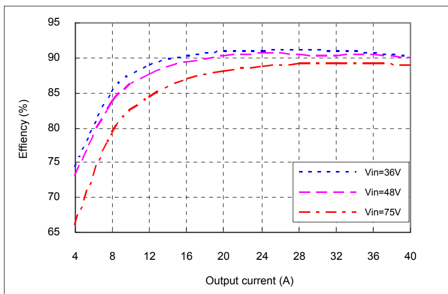
Figure 1 Efficiency vs. output current, T_a=25^{\circ}\text{C} , V_o=2.5\text{V}
