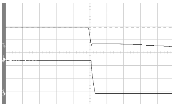
Figure 8 Output voltage shut down by power off, (5ms/div), see Figure 11 for test configuration; CH1-input voltage (50V/div); CH2-output voltage (1V/div)
