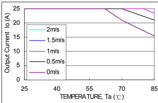
Fig.43 Output power derating AGQ100-48S1V5 (airflow direction from output to input, open frame)
