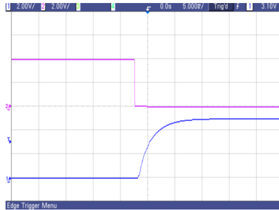
Fig.30 Typical start-up from CNT on of AVQ100B-48S05
