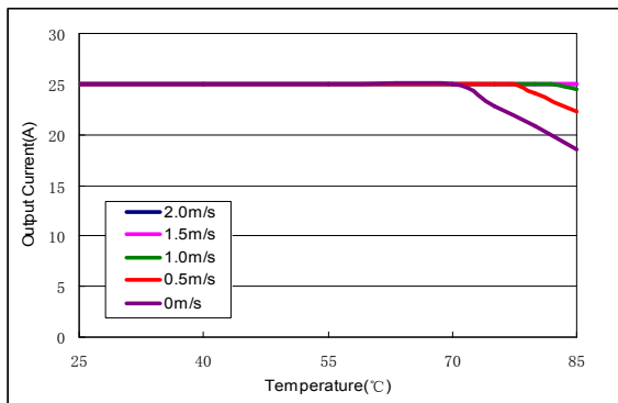
Fig.46 Output power derating AGQ100-48S1V8 (airflow direction from output to input, baseplate)
