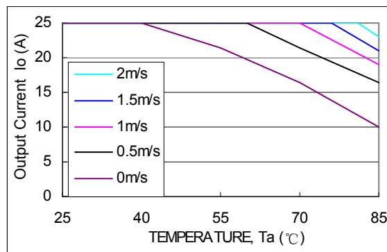
Fig.47 Output power derating AVQ100B-48S3V3 (airflow direction from output to input, open frame) Fig.48 Output power derating AVQ100B-48S3V3 (airflow direction from output to input, baseplate)
