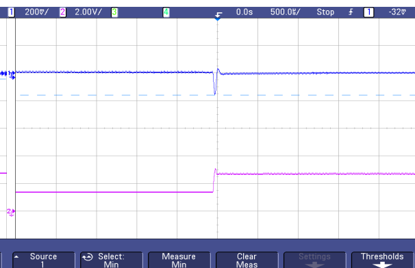
Fig.32 Typical transient response to step decrease in load from 50% to 25%, room temperature, 48Vdc input ( \Delta I_o/\Delta t = 1A/1\mu s ) of AGQ100-48S1V2
