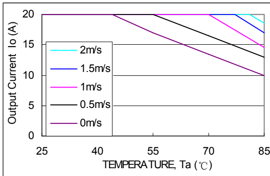
Fig.49 Output power derating AVQ100B-48S05 (airflow direction from output to input, open frame) Fig.50 Output power derating AVQ100B-48S05 (airflow direction from output to input, baseplate)
