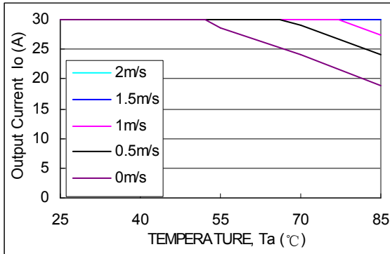
Fig.41 Output power derating AGQ100-48S1V2 (airflow direction from output to input, open frame)
