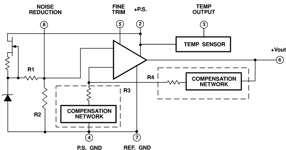
Figure 1. BLOCK DIAGRAM
