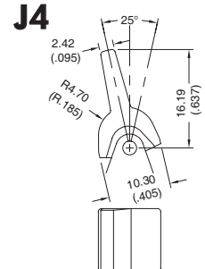
J4 Lever
