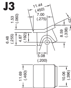
J3 Rocker
