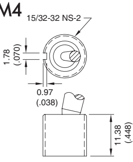
15/32" threaded
