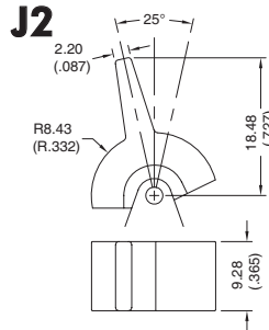
J2 Lever
