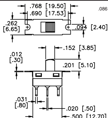
MECHANICAL OUTLINE
