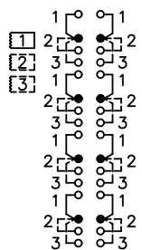
SCHEMATIC
