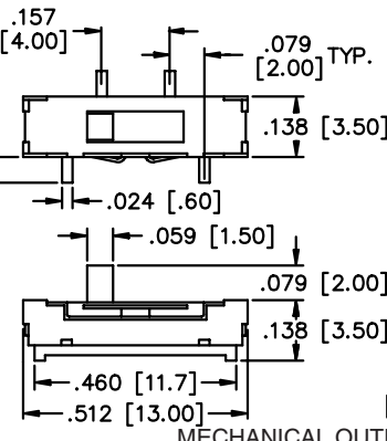
MECHANICAL OUTLINE
