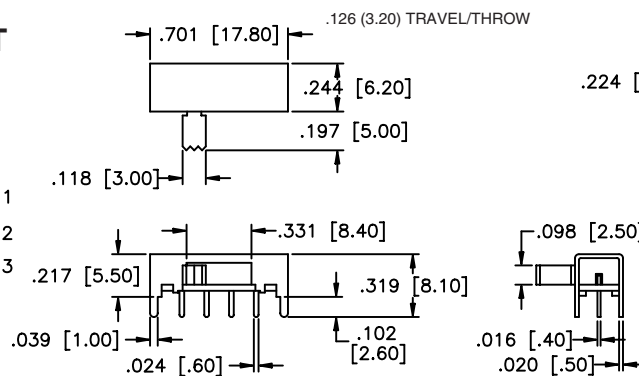
MECHANICAL OUTLINE
