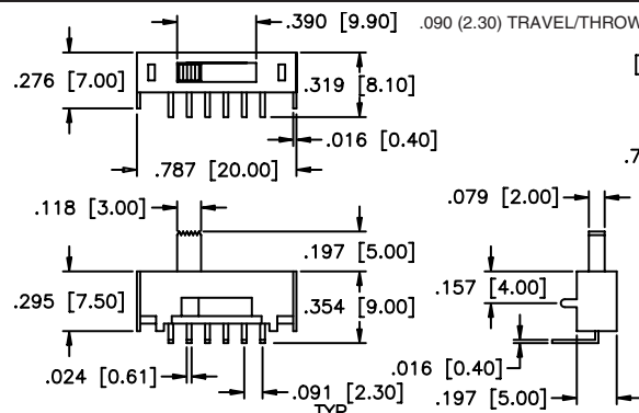
MECHANICAL OUTLINE
