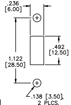
PANEL CUTOUT
