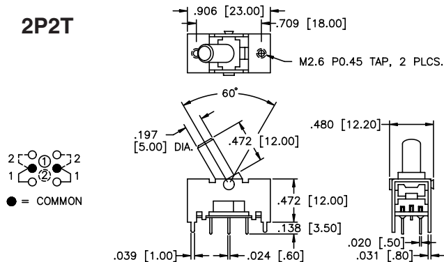
SCHEMATIC
