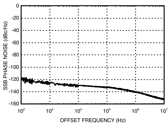
SSB Phase Noise Performance, F_{out} = 27 \text{ GHz} , P_{in} = 0 \text{ dBm}
