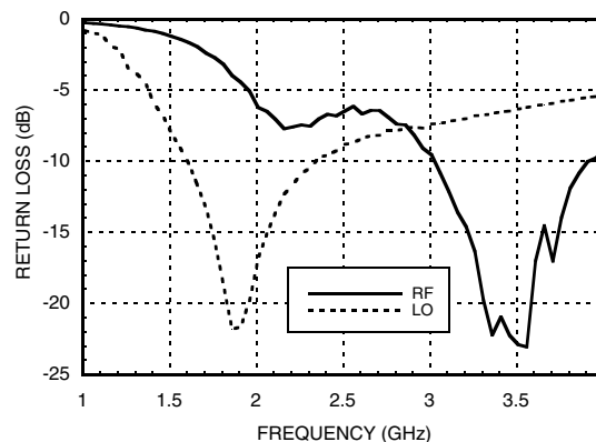
Return Loss @ LO = +10 dBm
