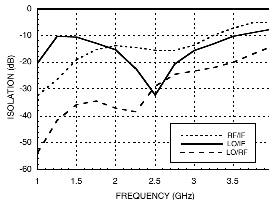
Isolation @ LO = +10 dBm
