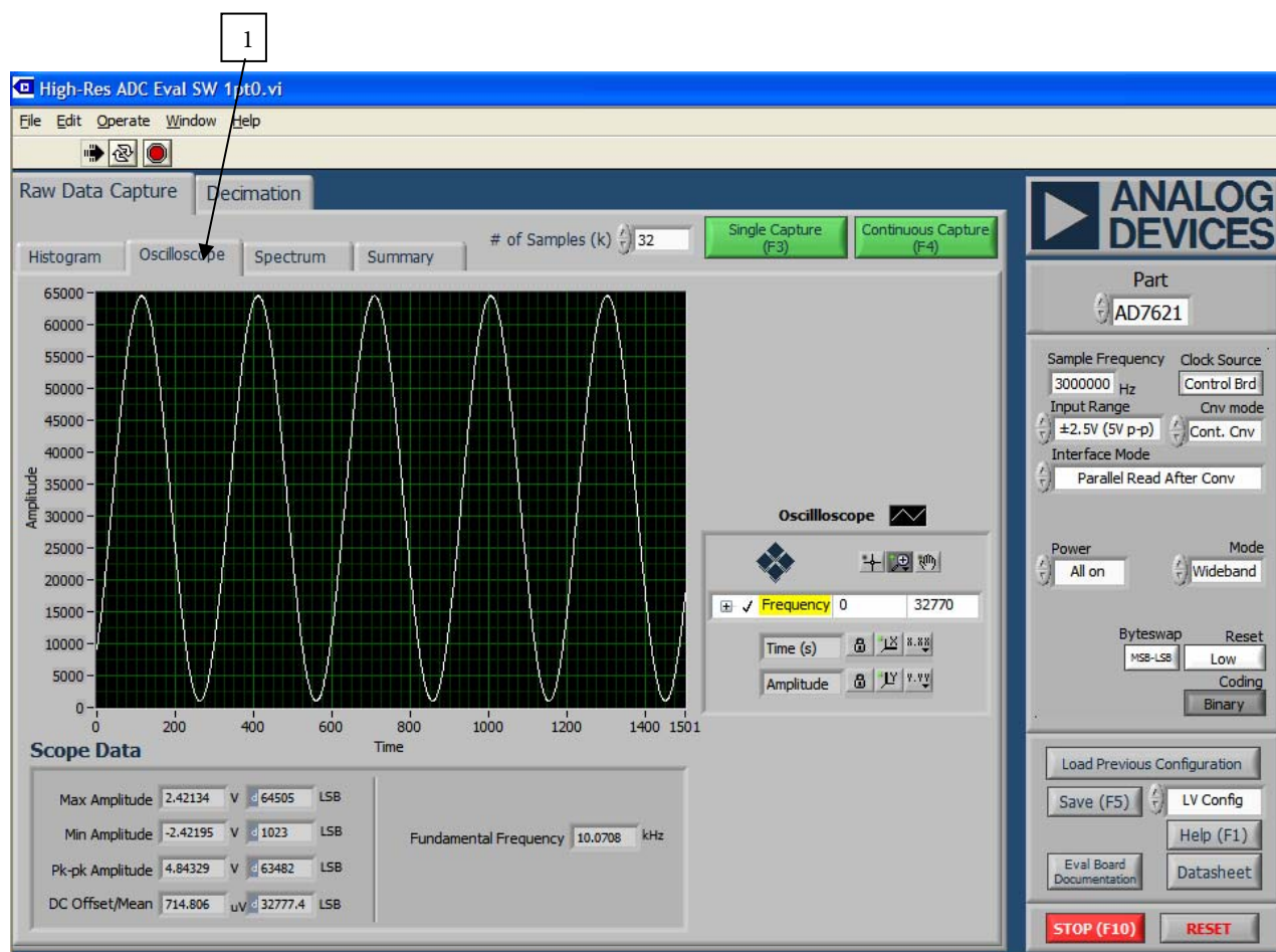
Figure 16. Oscilloscope
