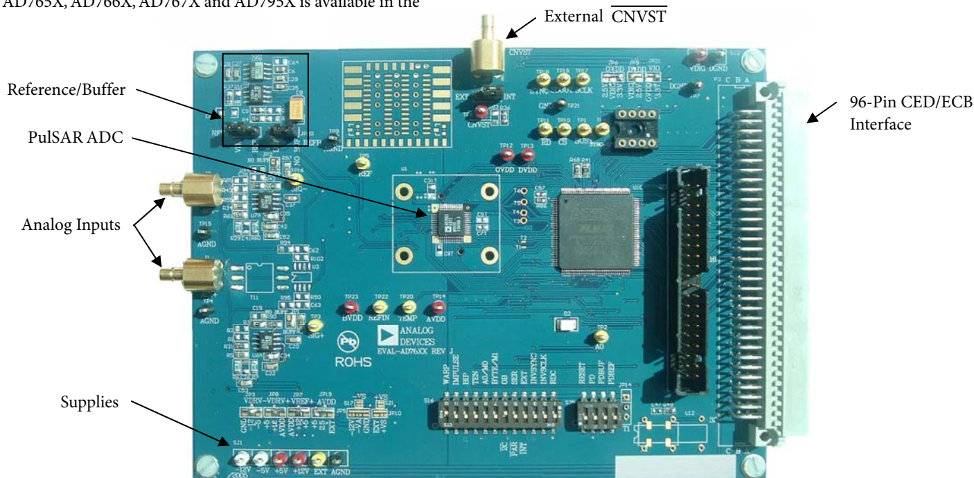
Figure 1. Evaluation Board
