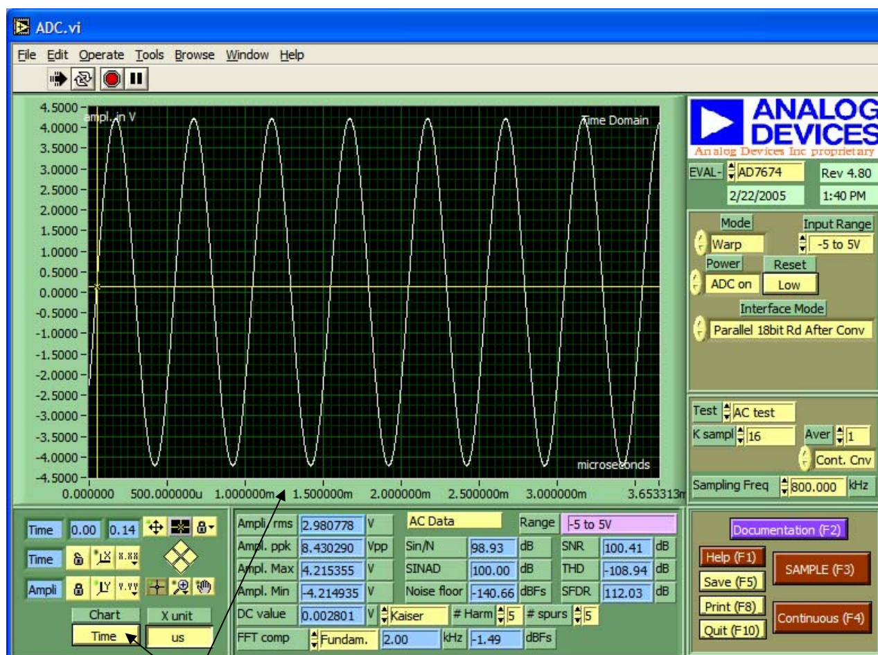
Figure 21. Time-Domain Screen
