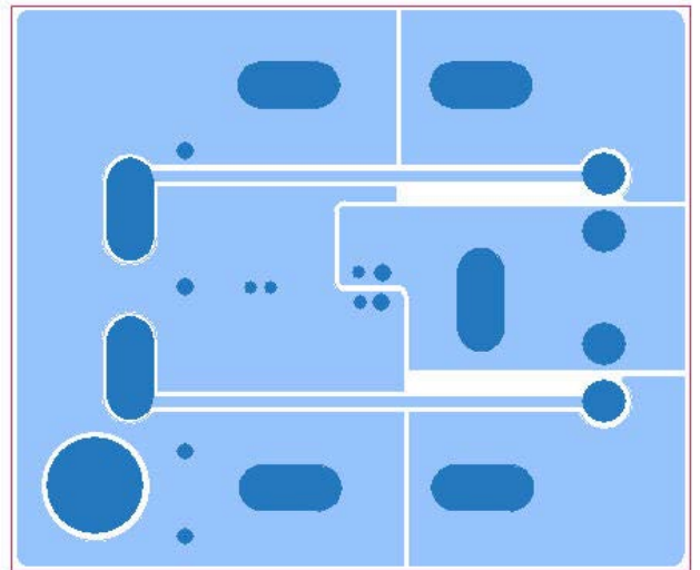
Figure 41. Example of PCB Layout, Bottom Side
