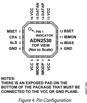
Figure 4. Pin Configuration
