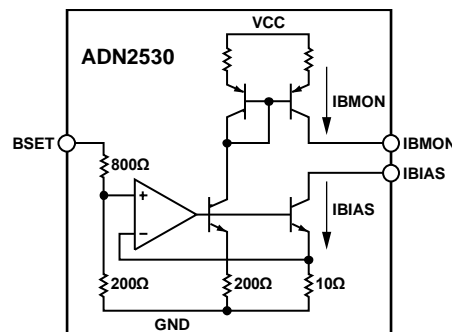
Figure 24. Voltage-to-Current Converter Used to Generate IBIAS
