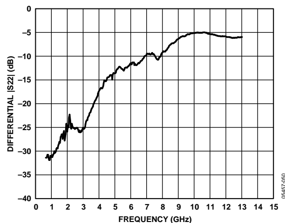
Figure 10. Differential |S_{22}|
