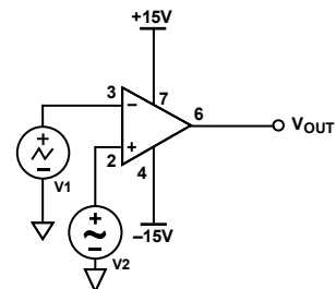
Figure 54. Pulse-Width Modulator
