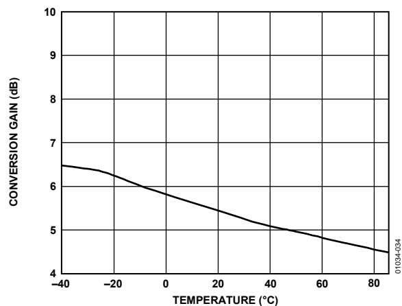
Figure 34. Gain Performance Over Temperature; f_{IN} = 2400 MHz, f_{OUT} = 425 MHz
