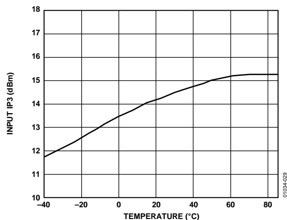
Figure 29. Input IP3 Performance Over Temperature; f_{IN} = 2400 MHz, f_{OUT} = 170 MHz
