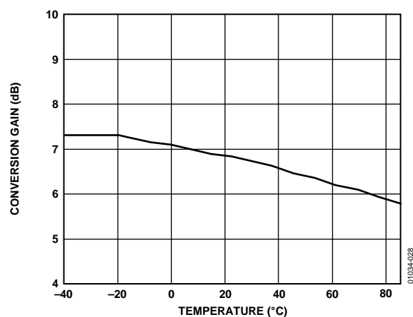
Figure 28. Gain Performance Over Temperature; f_{IN} = 2400 MHz, f_{OUT} = 170 MHz
