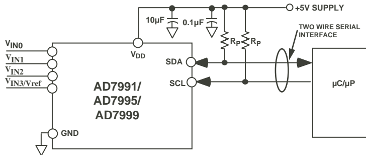
Figure 24. AD7991/AD7995/AD7999 Typical Connection Diagram
