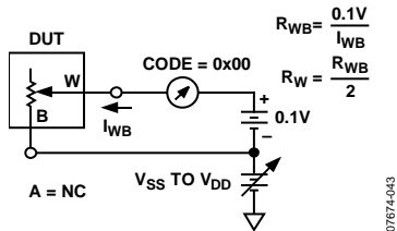
Figure 60. Wiper Resistance
