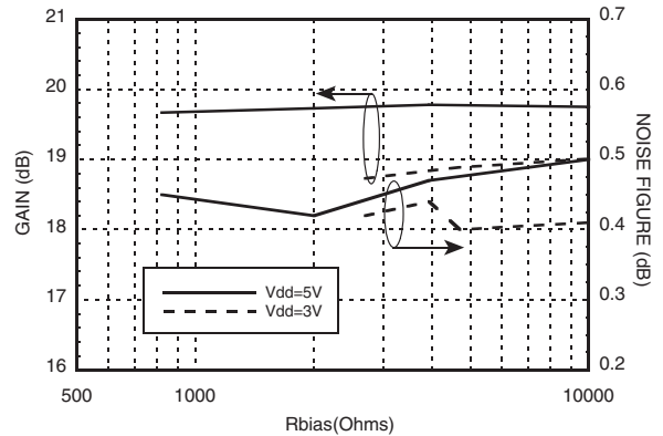
Gain, Noise Figure & Rbias @ 500 MHz
