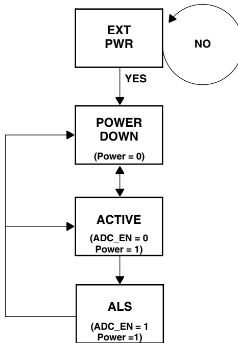
Figure 5. State Diagram
