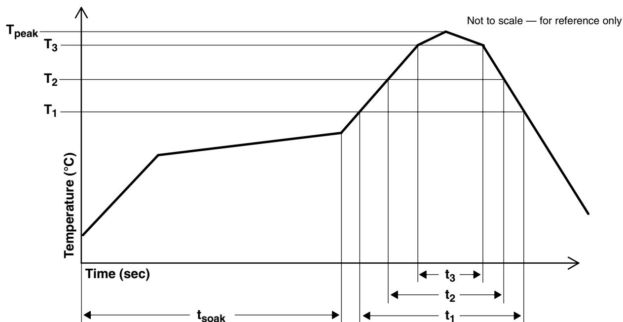
Figure 13. Solder Reflow Profile Graph
