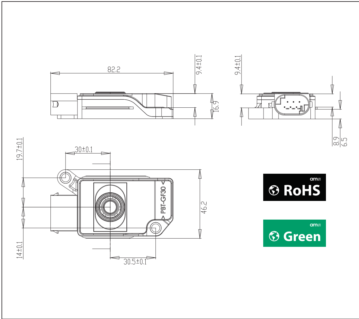
Figure 17: Sensor Dimensions
