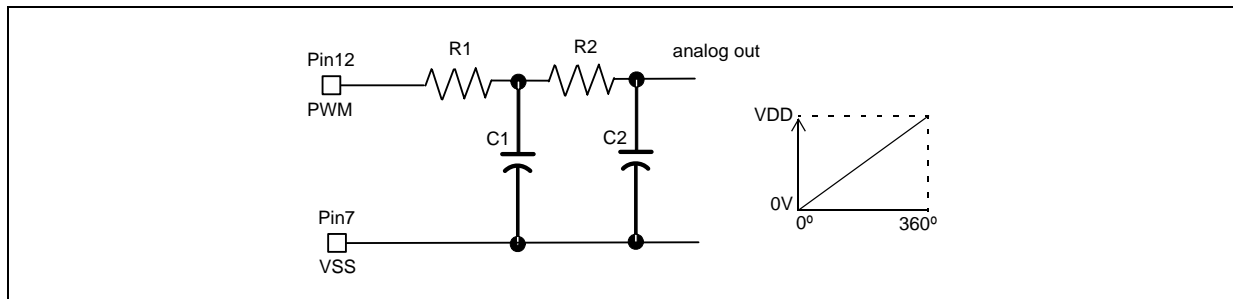
Figure 11: Simple 2nd order passive RC low pass filter
