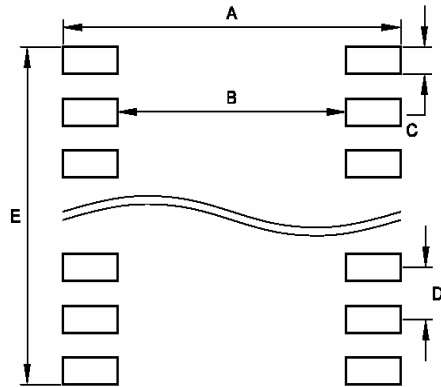
Figure 24. PCB Footprint
