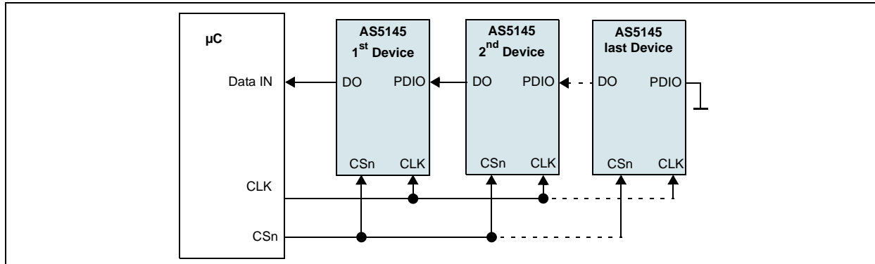
Figure 9. Daisy Chain hardware configuration
