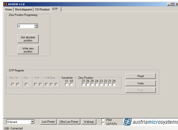
Figure 5: OTP tab
