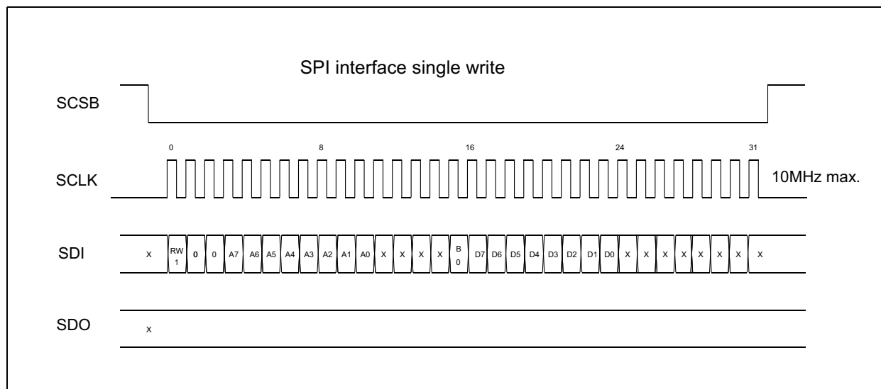
Figure 81: SPI Single Write
