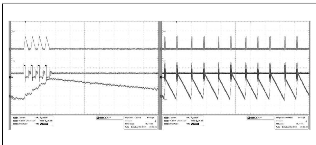
Figure 14: DC/DC Buck Dis-Continuous Mode & High Efficiency 2/2
