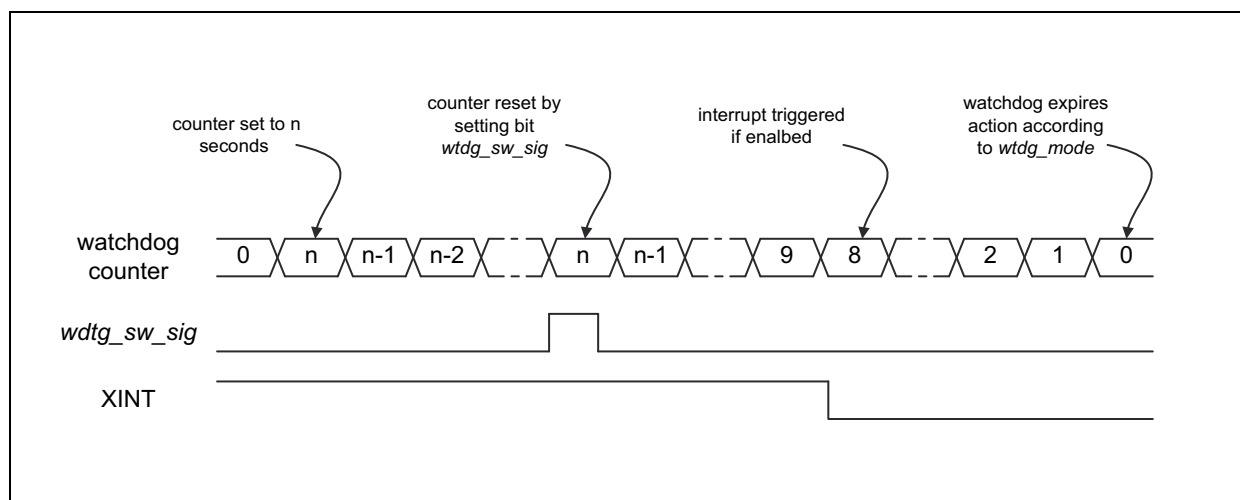
Figure 68: Watchdog Timing
