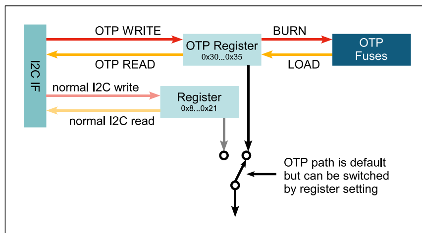
Figure 17. Register Access
