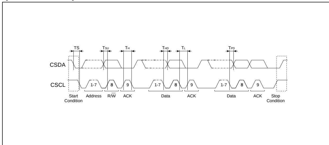
Figure 26. 2-Wire Serial Timing
