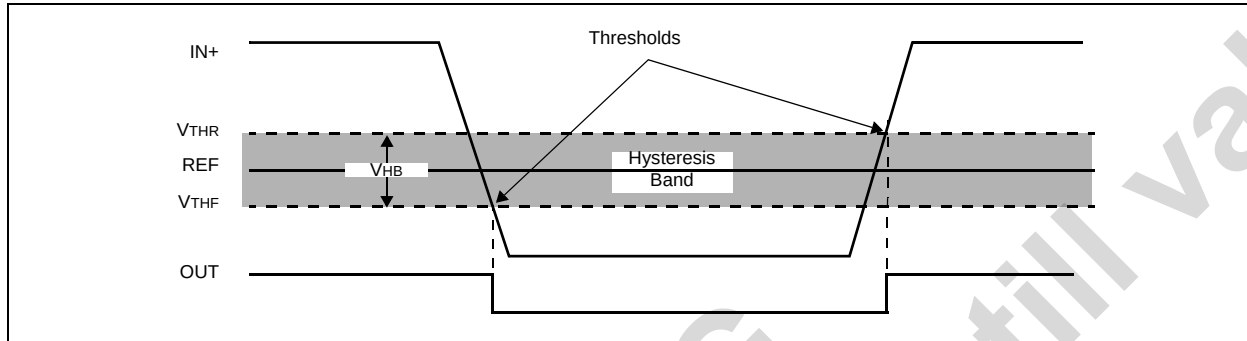
Figure 20. Threshold Hysteresis Band
