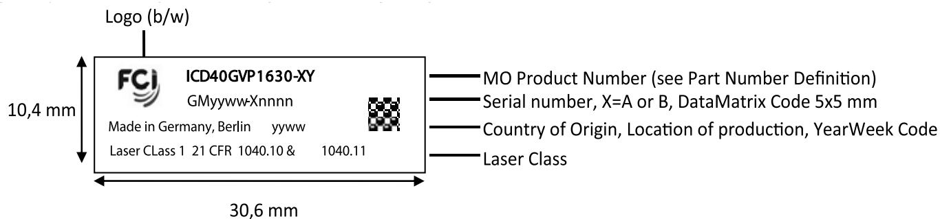
Figure 11 Label Position on Bottom Side of Housing
