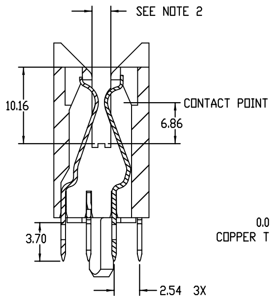
SECTION X-X
