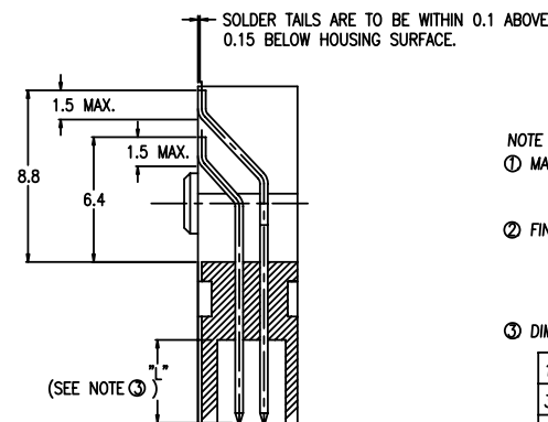
SECTION "E-E" (5/1)
