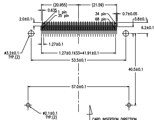
CARD INSERTION DIRECTION RECOMMENDED FOOT PRINT (MOUNTED SIDE)
