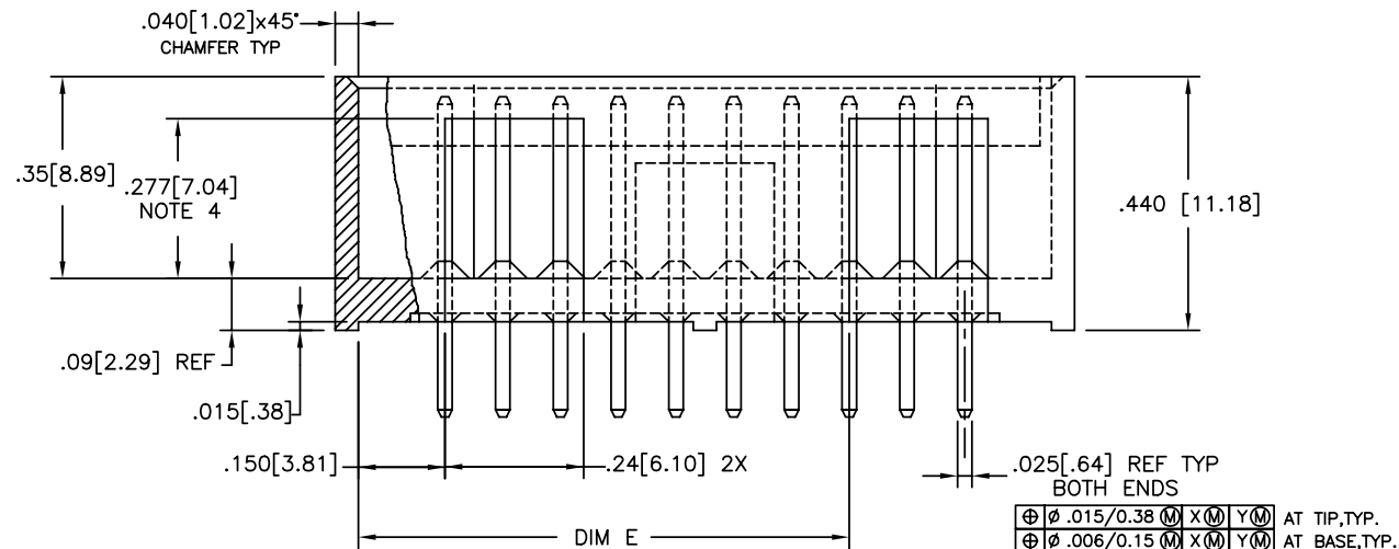
VIEW G-G
