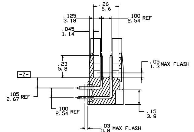
SECTION G-G ROTATED 90° CW
