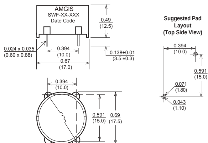
Type "F" - Flat Mount - Size 2
