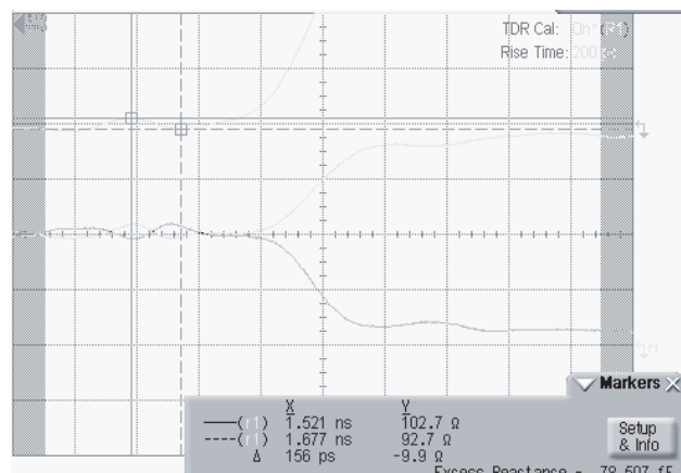
Figure 12. 140Ω Differential Impedance with AOZ8006 MSOP-10 Package on it Max. 102Ω, Min. 92Ω
